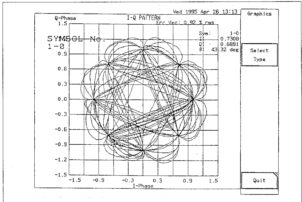
図1-4 I-Q diagram (20 point)
