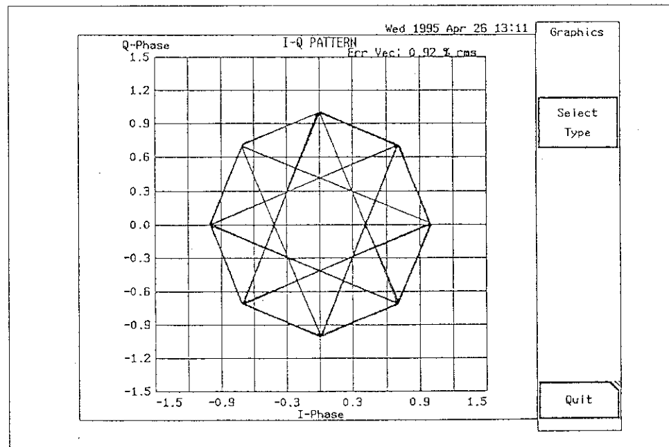
図1-3 I-Q diagram (Linear)
