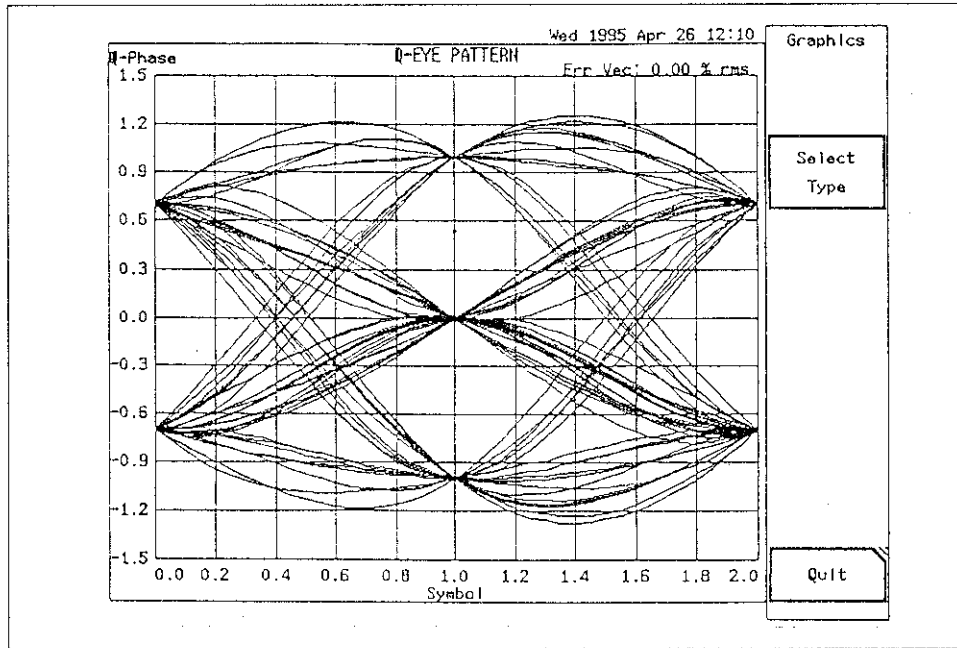
図1-6 Q channel EYE diagram
