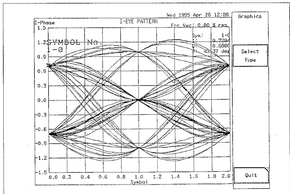
図1-5 I channel EYE diagram
