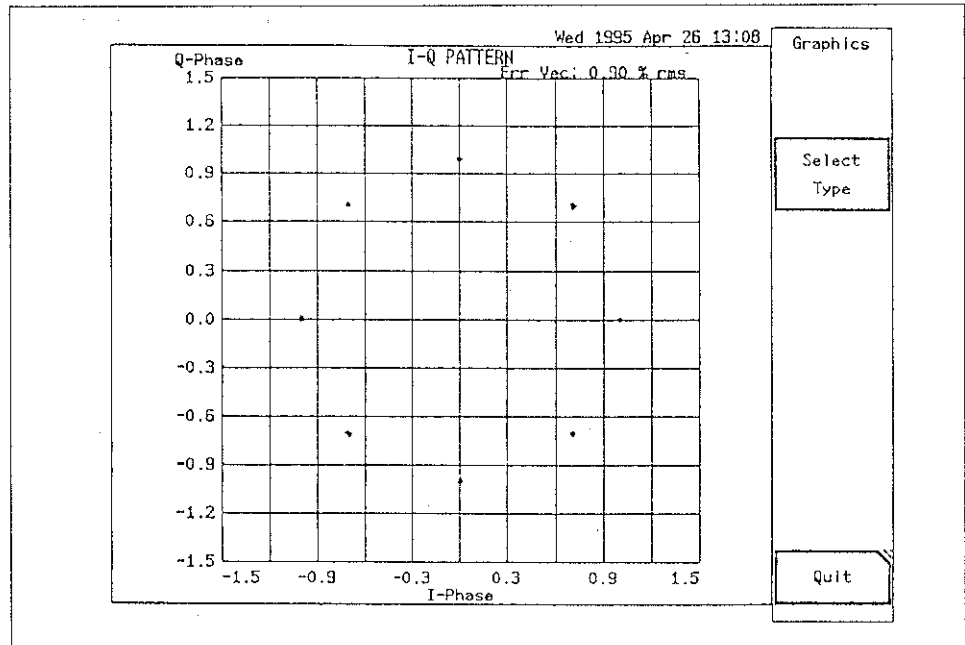
図1-2 I-Q diagram (Non-interpolate)
