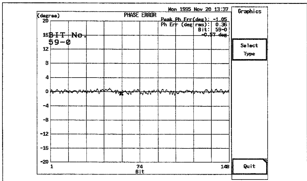
図1-3 Phase Error
