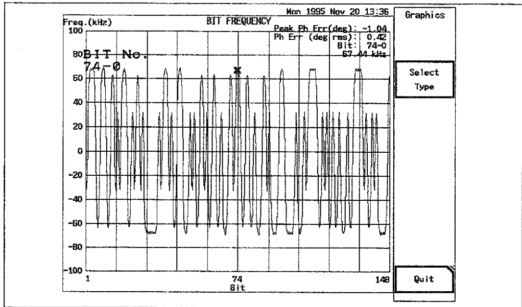
図1-2 Bit-Frequency
