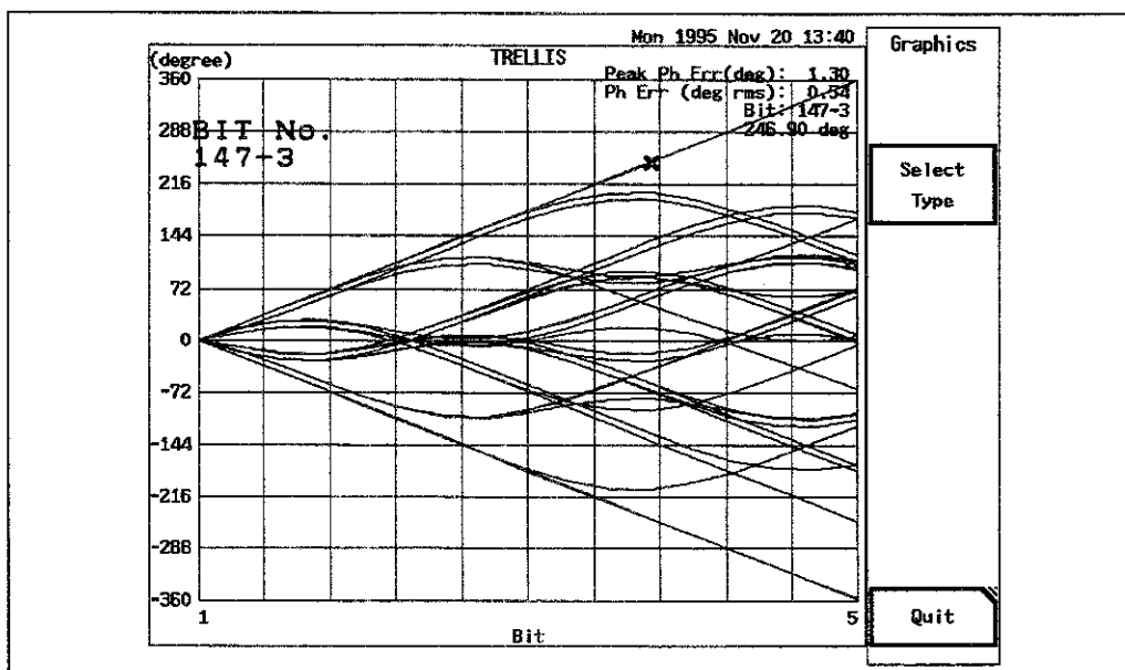
図1-5 Trellis
