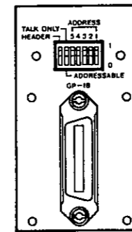
GP-IB PANEL
